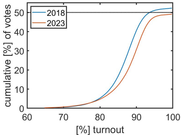
FIG. 1: Votes for Erdogan as a function of voter turnout for 2018 and 2023. For a given turnout level, the cumulative vote share of ballot boxes with this or lower turnout is shown. In 2018, a majority of more than 50% is achieved by including boxes with a turnout of more than 90%. In 2023 (red line) we observe similar characteristics with higher turnout and lower vote shares (below 50%).
