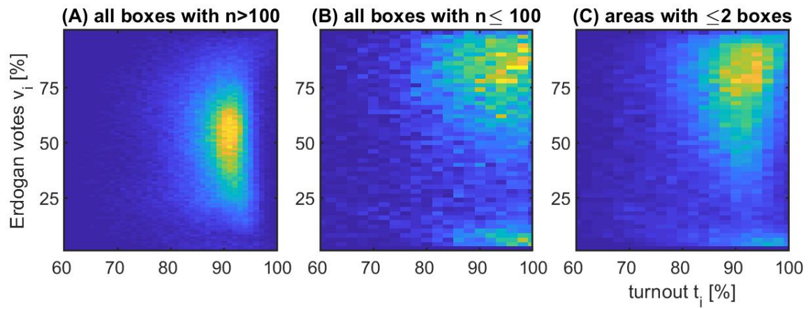
FIG. 4: The fingerprints in 2023 for small units (B,C) show very different patterns than those with an electorate size of more than 100 (A). Considering only areas with an electorate size of less than 100 (B), or alternatively ballot boxes from areas with one or two ballot boxes (C), results in a bimodal distribution with a large mode in the region with very high turnout and votes for Erdogan.
